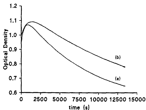
Figure 1. Variation of O. D. vs Time for the Ammonolysis of 1 at 13.5°C in (a)=3.72 M, (b)= 2.26 M \text{NH}_3 .
