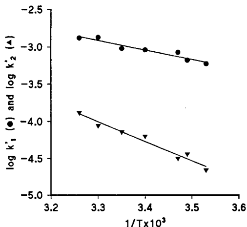
Figure 4. Plot of \log k'_1 and k'_2 vs. 1/T for ammonolysis of 1 and 2 , respectively.
