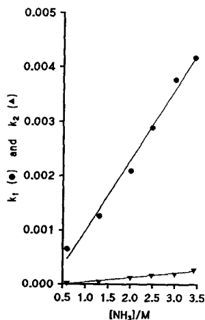
Figure 3. Dependence on \text{NH}_3 concentration of k_1 and k_2 for kinetics performed at 30°C.
