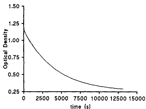
Figure 2. Variation of O. D. vs Time for the Ammonolysis of 2 at 21°C in 3.8 M \text{NH}_3 .
